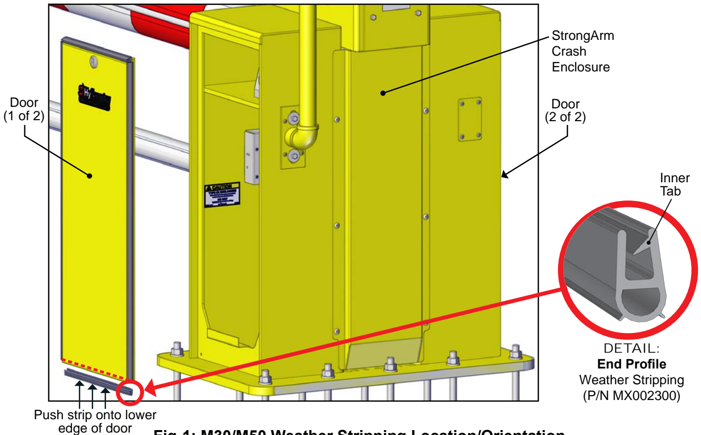
Fig-1: M30/M50 Weather Stripping Location/Orientation
