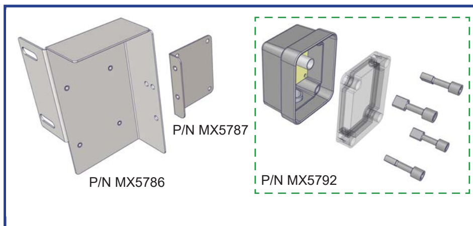
FIG-1: P/N MX5803, NEW PhotoEye Enclosure Kit
