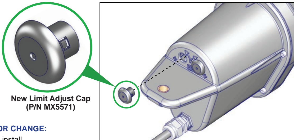
FIG-1: Nice 816 Actuator Limit Switch Adjust Cap Location
