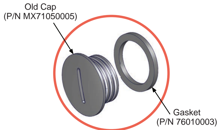
FIG-2: Old Limit Adjust Cap & Gasket
